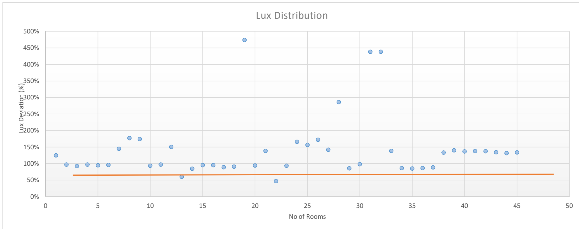
Figure 7: Room luminance survey at CIO’s Office (ARAS ATAS)
