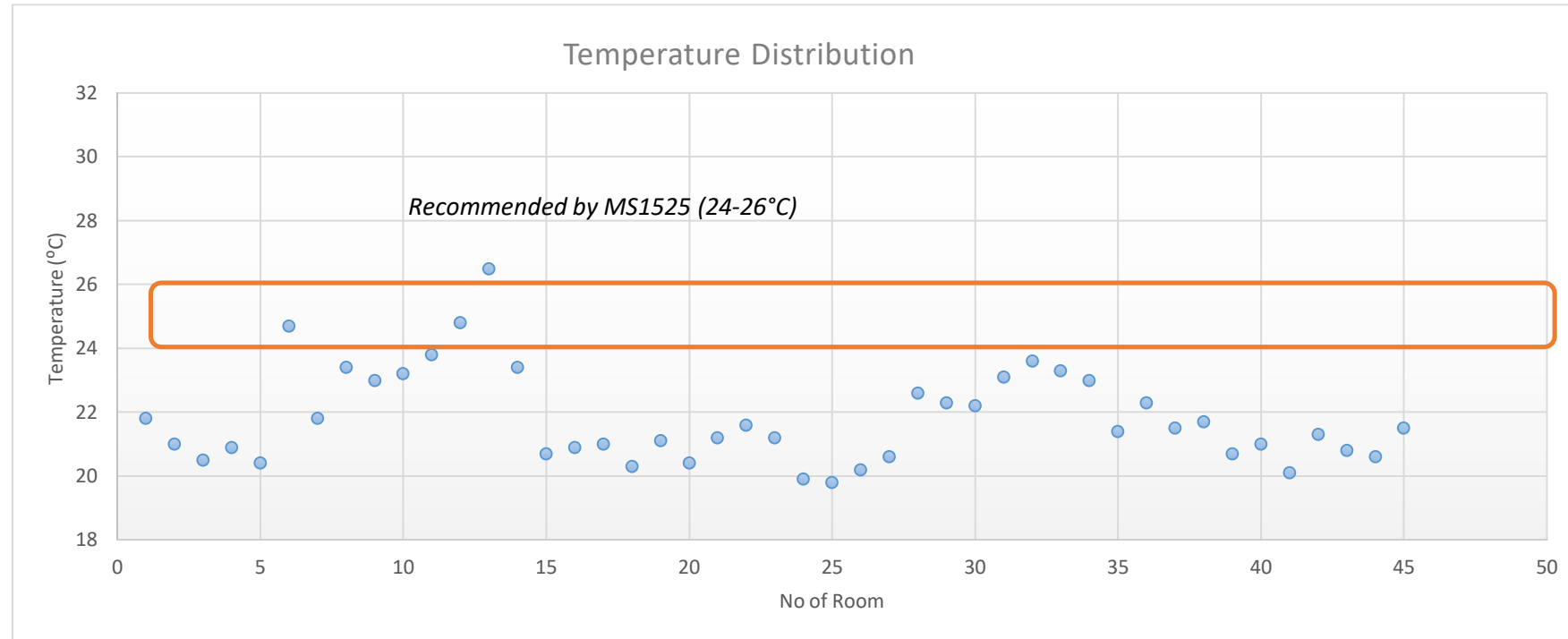
Figure 1: Room temperature survey at CIO's Office (ARAS ATAS)
