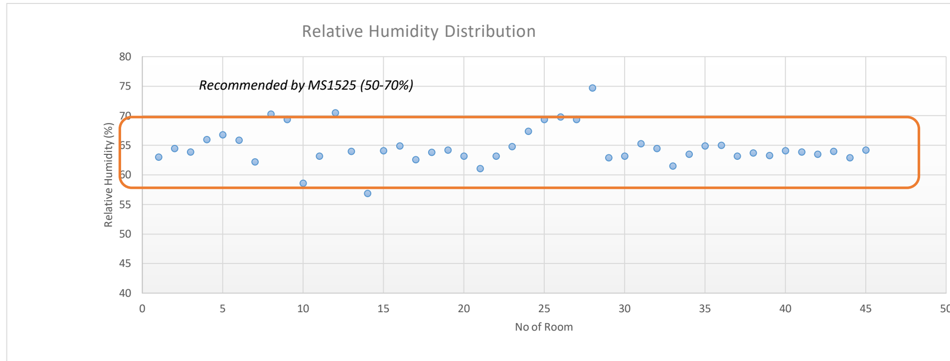
Figure 3: Room relative humidity survey at CIO's Office (ARAS ATAS)
