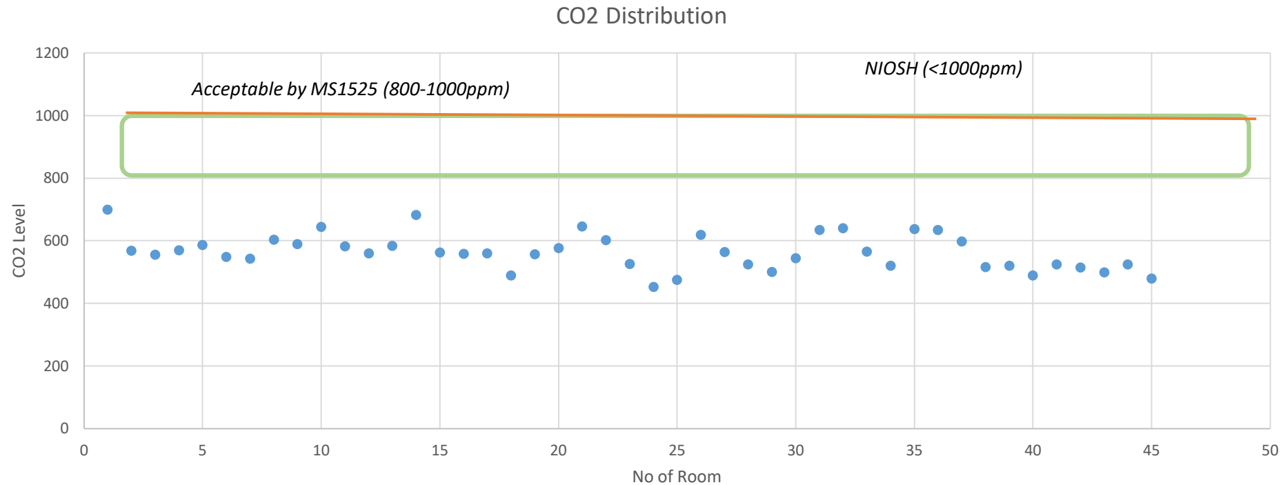
Figure 5: Room carbon dioxide survey at CIO's Office (ARAS ATAS)
